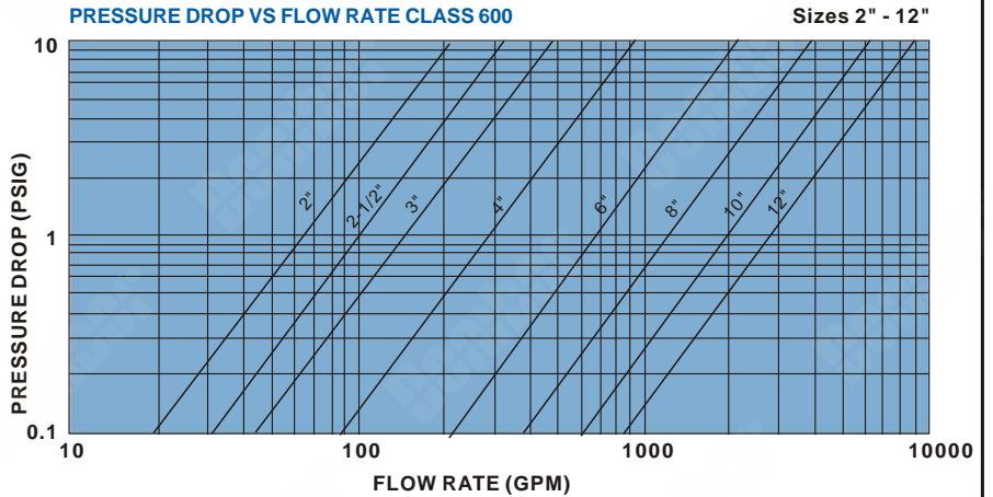
PRESSURE DROP VS FLOW RATE CLASS 600
